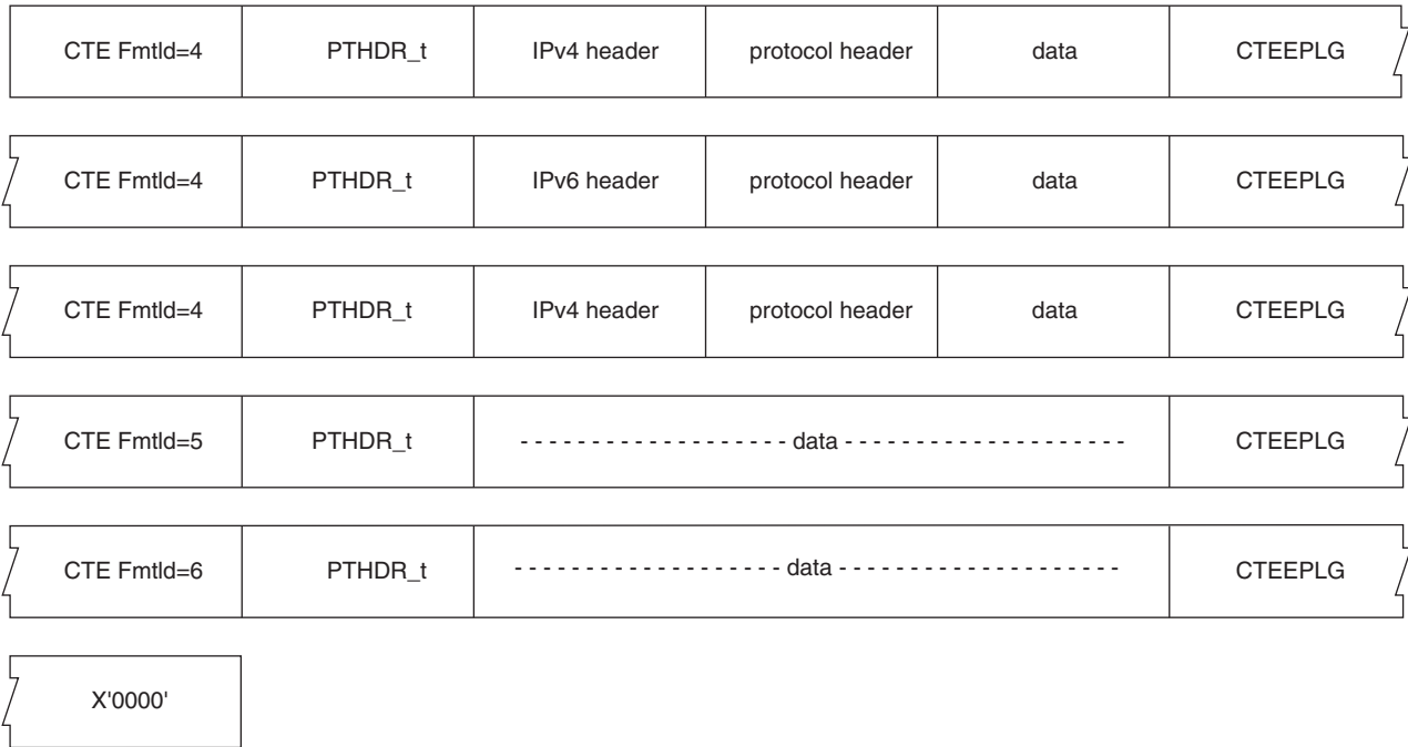
Figure 31. CTE layout
