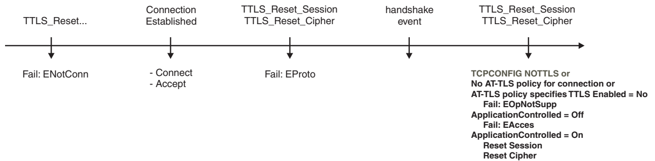
Figure 34. SIOCTTLCTL with TTLS_Reset_Session or TTLS_Reset_Cipher
