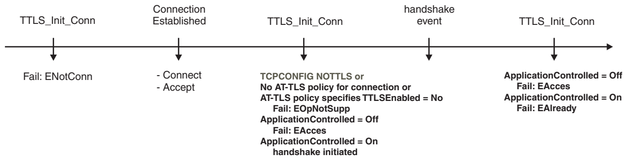
Figure 33. SIOCTTLCTL with TTLS_Init_Connection
