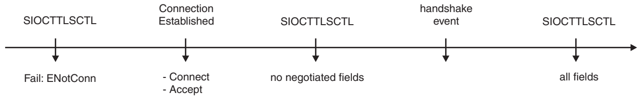
Figure 32. SIOCTTLCTL with TTLS_Query_Only
